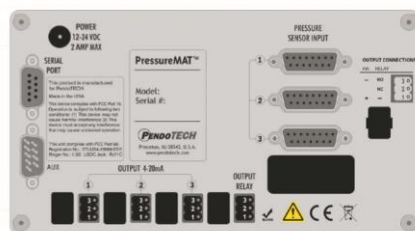
Illustration: Back panel schematic of PMAT3
